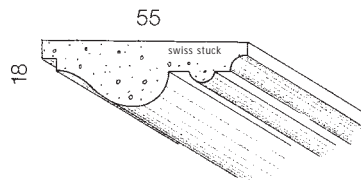
▲ P051 18×55mm
