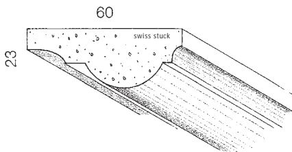
▲ P062 23×60mm ▲ P061 30×80mm
